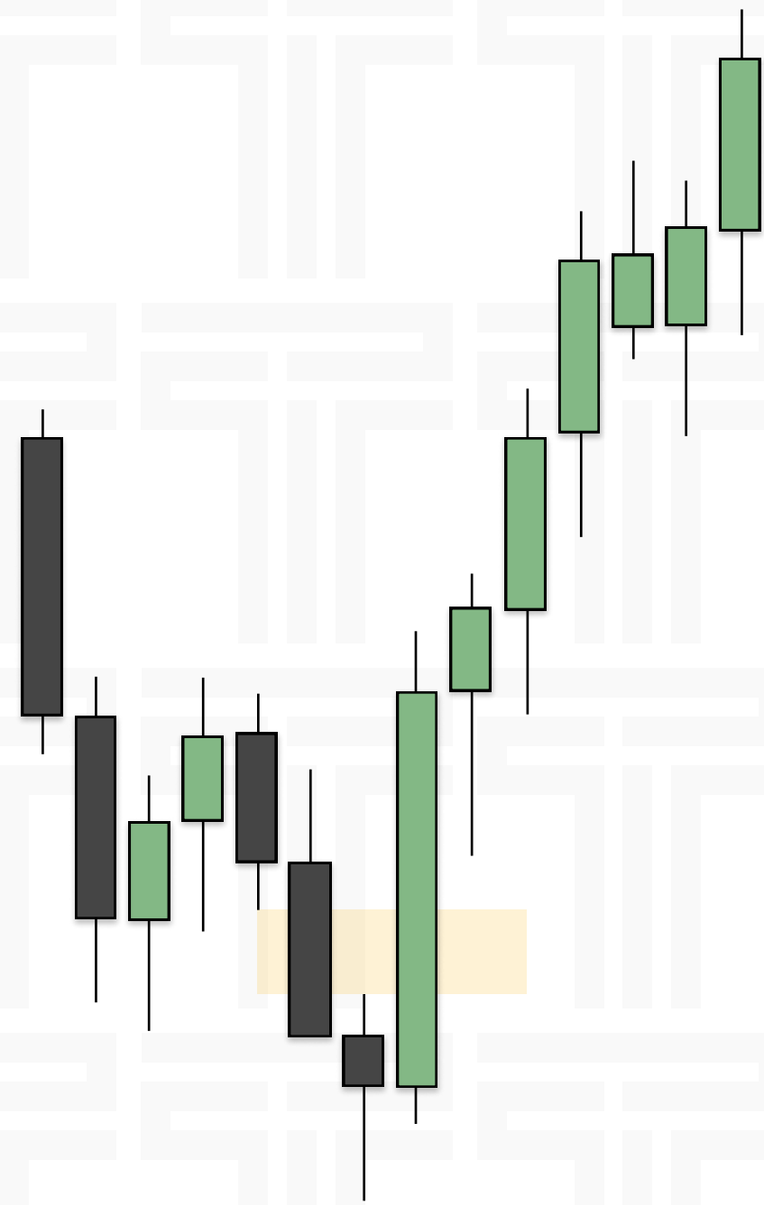
Bullish IFVG
