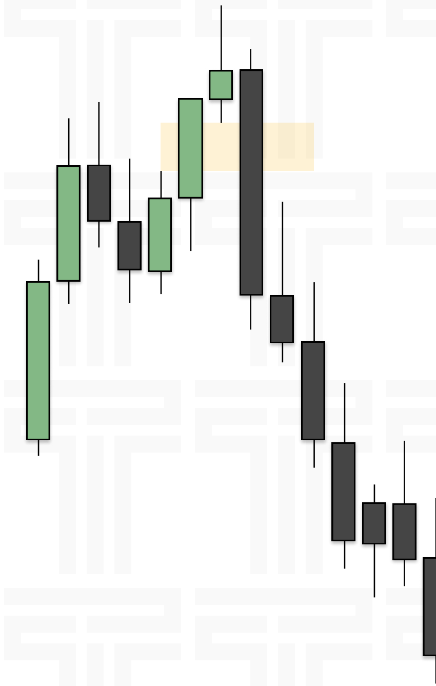
Bearish IFVG
