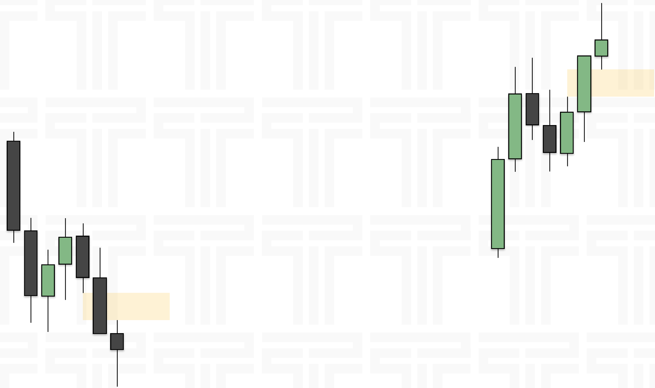
Bearish FVG
